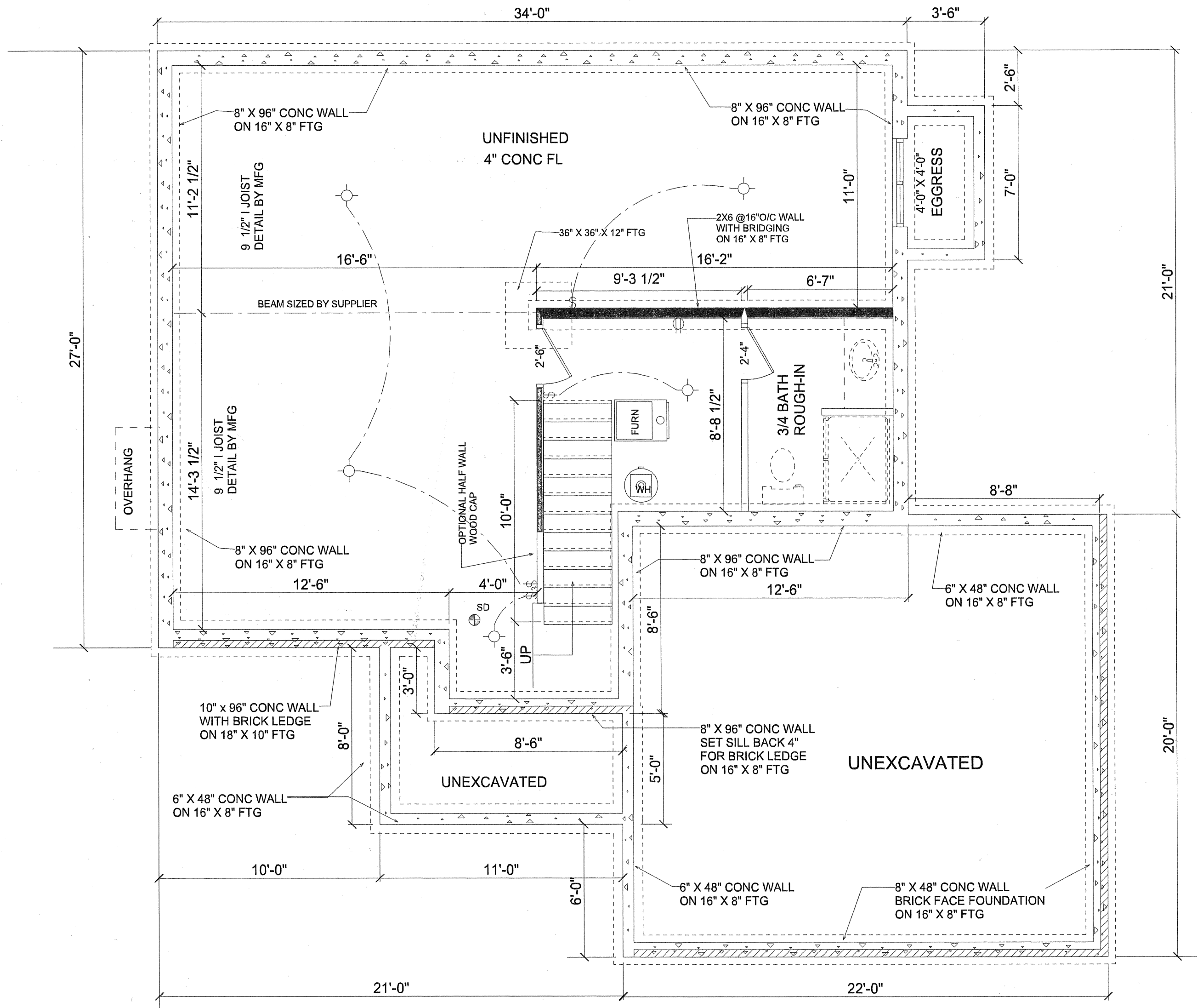
FOUNDATION 791 UNFISHED SQ.FT. SCALE 1/4" = 1'-0"
