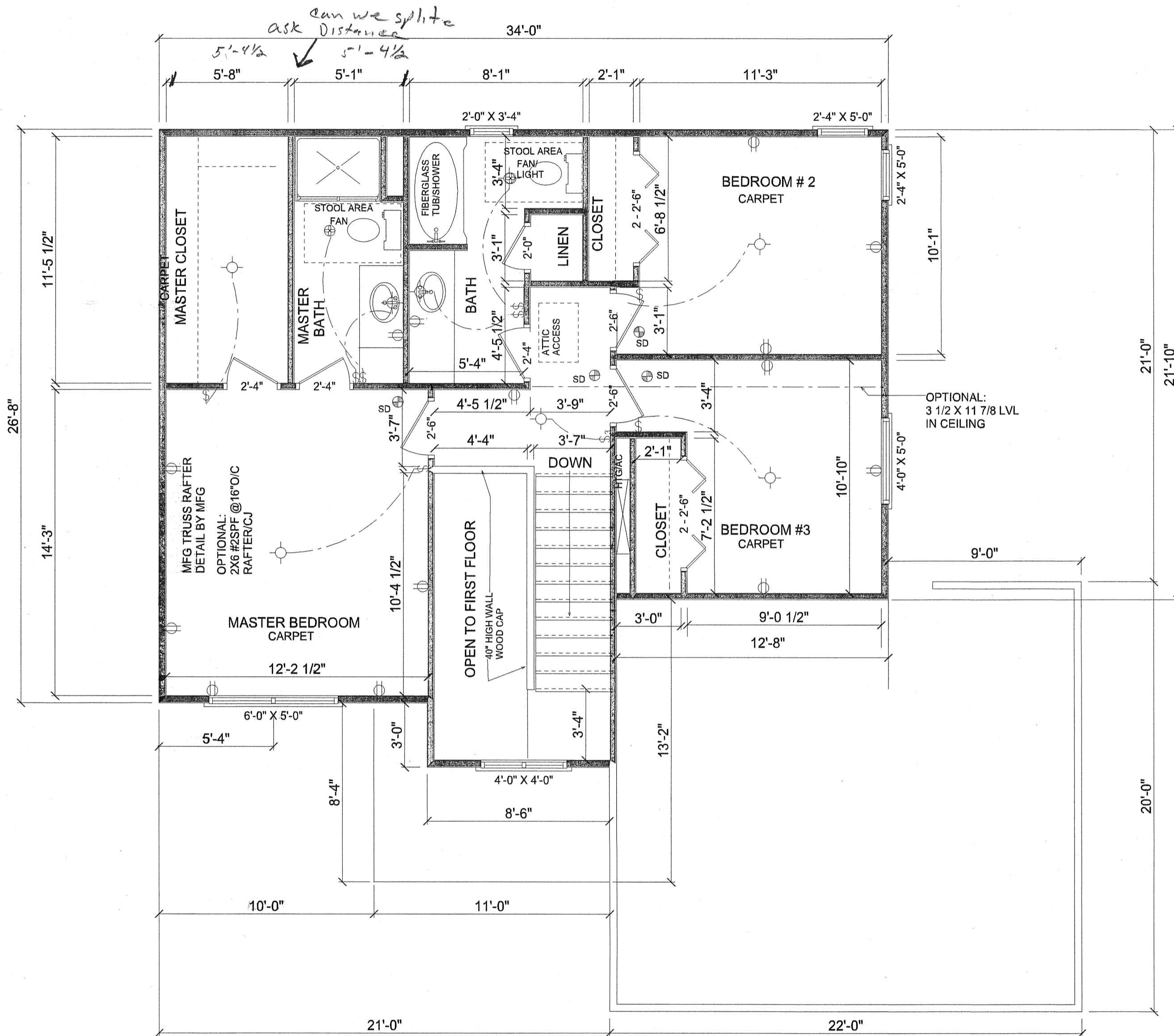
SECOND FLOOR 762 SQ. FT SCALE 1/4" = 1'-0"
